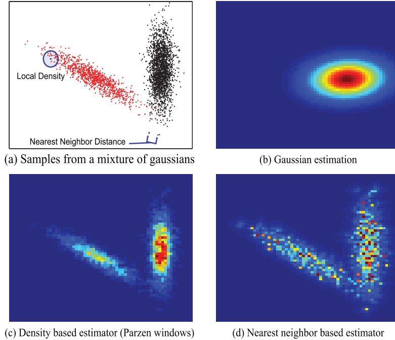
Figure 16. A comparison of density estimators. The upper left figure illustrates a multi-modal data distribution and two methods of non-parametric density estimates. On the upper right the image represents a gaussian density estimate, which does not fit the data well. The lower left image shows the estimate from Parzen windowing and the lower right image shows an estimate based on the K-L nearest neighbor approach.
