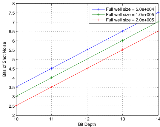
Figure 2. The three curves represent the shot noise in bits as a function of bit depth for three different full well values.
