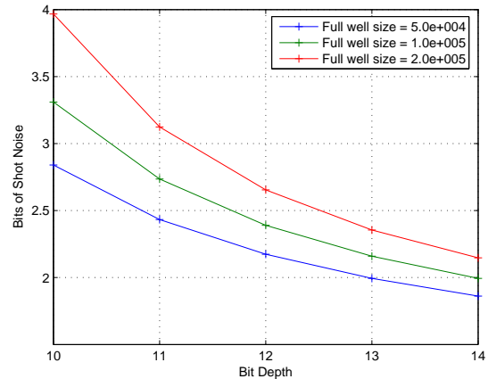
Figure 3. The three curves represent the compression ratio for pure shot noise in bits as a function of bit depth for three different full well values.
