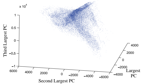
Figure 15. A scatter plot of the 10 \times 10 window of the 11 spectral channels ABI-proxy data projected into the first three principal components.
