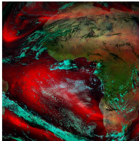
Figure 1. A false color image combining information from the 11 channels of the 12 channel Meteosat-8 imager. The red swirls show data from the water vapor channels.
