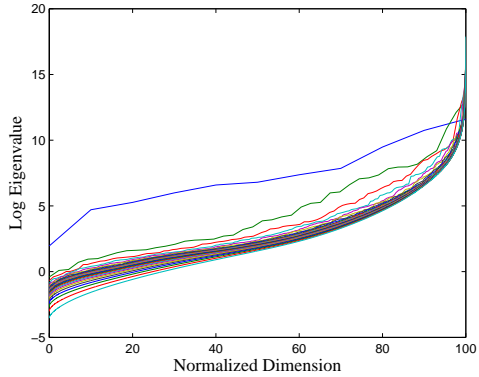
Figure 10. Rescaled log-eigenvalue curves for windowed ABI-proxy data. Spatial window sizes ranging from a single footprint (with all channels) to 25 \times 25 are shown as different curves. The curves converge as the window sizes increase.
