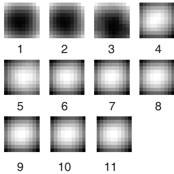
Figure 5. The first principal component of windowed ABI-proxy data as 11 normalized images of size 10 \times 10 .
