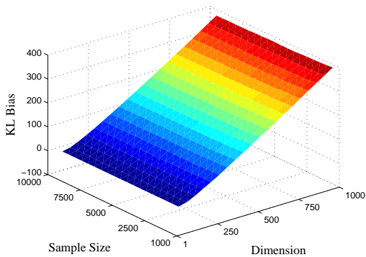
Figure 17. Surface showing the bias for K-L entropy estimator applied to an isotropic unit gaussian distribution as a function of dimension and sample size. Even though the bias vanishes with increasing sample size, the bias shrinks very slowly.
