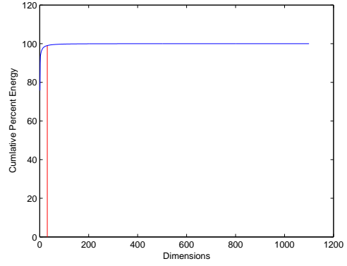
Figure 9. Graph showing the percentage of the total variance explained by subspaces. Note that 99% of the variance is explained by just 43 out of the 1100 dimensions.
