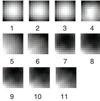
Figure 6. The second principal component of windowed ABI-proxy data. Both the first and second principal components show a dominant variation in the spectral dimensions.
