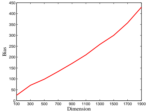
Figure 19. A plot showing the bias in entropy remaining after applying our bias corrected K-L estimator applied to known distributions as a function of dimensions applied to a validation set.
