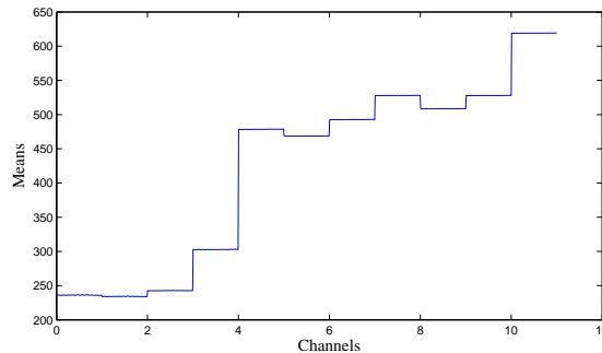
Figure 4. The mean of 10 \times 10 spatial windows of footprints (all channels) of the ABI-proxy data. Note that the mean is constant within each channel.
