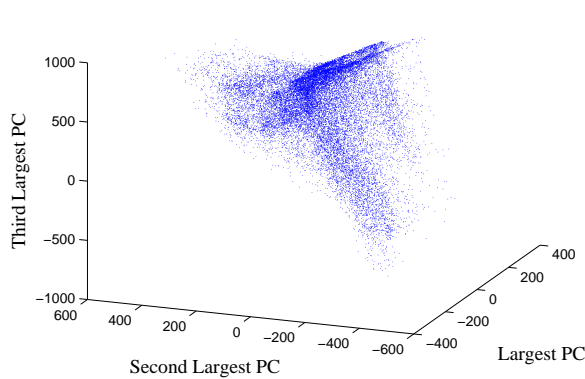
Figure 14. A scatter plot of the 11 spectral channels ABI-proxy data projected into the first three principal components.
