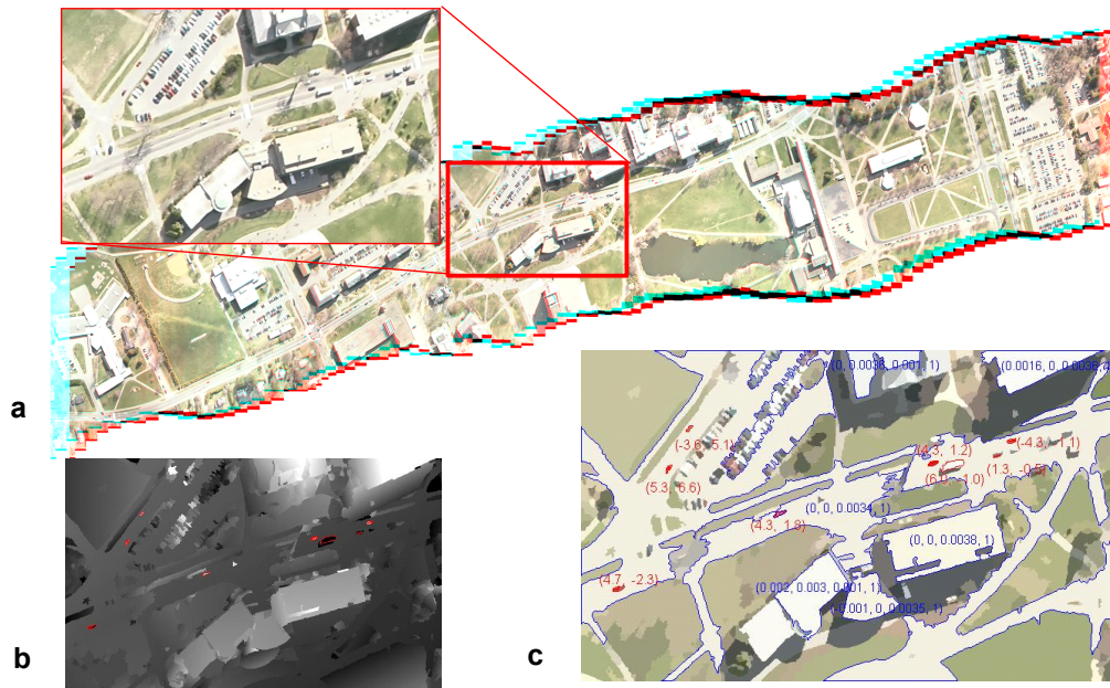
Fig 4. Content-based 3D mosaic representation of an aerial video sequence. (a) A pair of stereo mosaics from the total nine mosaics and a close-up window; (b) the height map of the objects inside that window; (c) the CB3M representation with some of the regions labeled by their boundaries and plane parameters (in blue), and the detected moving targets marked by their boundaries and motion vectors (in red).
